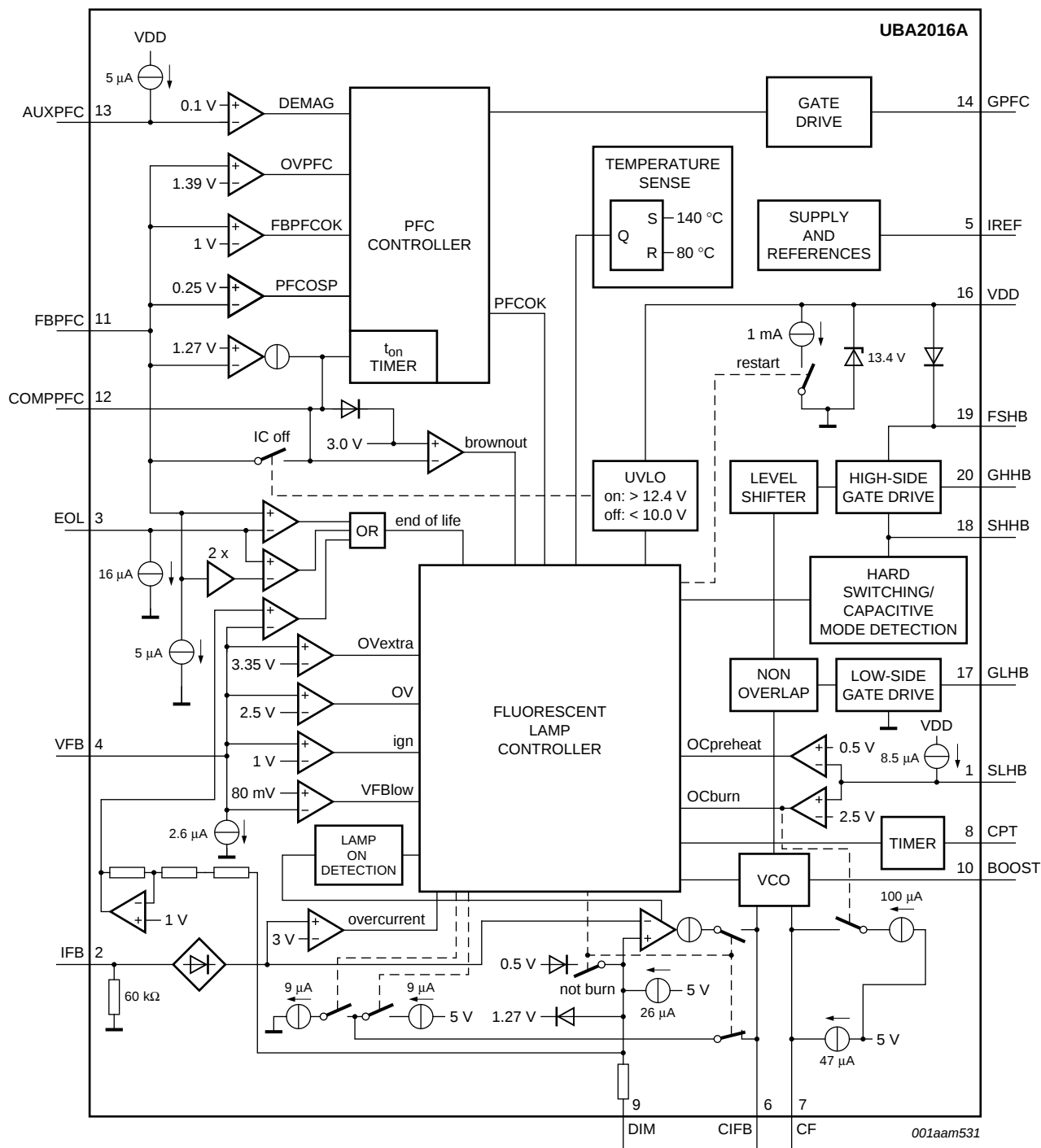
Fig 1. Block diagram UBA2016A
